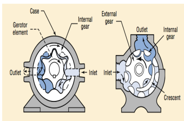
Fig 2: Gear Pump
