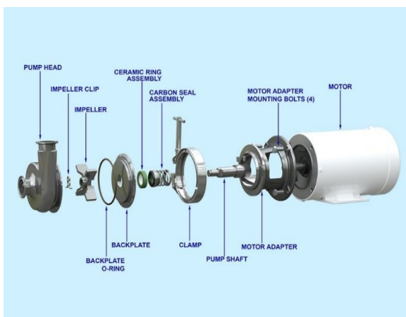
Fig 1: Essential Parts of Centrifugal Pump
